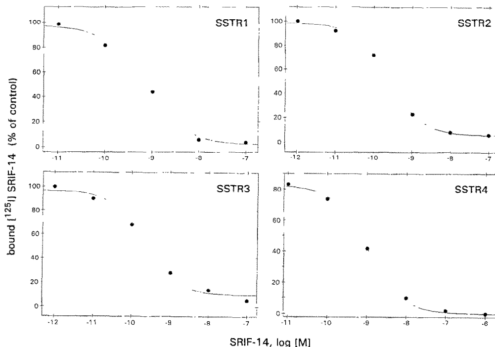
Fig. 3. Expression of SRIF receptor subtypes in HEK 293 cells. Concentration dependence for the inhibition of [ 125 I]-Tyr 11 -SRIF-14 binding by unlabelled SRIF-14. Results are expressed as percentage of maximal specific binding in the absence of competitor. The non-specific binding was less than 20% of the total binding.
